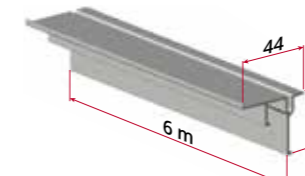
art. 2002 Binario inferiore in alluminio Aluminium lower rail
