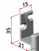
art. 3887 Guida inferiore in metallo per canalina art. 3525 Metal lower guide for art. 3525
