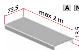
Art. 2009 Rivestimento a scatto in metallo per anta esterna Clicking metal cover for external door
