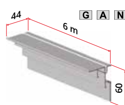
art. 2062 Profilo inferiore in alluminio con zoccolo H 60 mm Aluminium lower profile with wainscot H 60 mm
