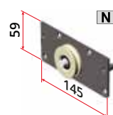
Art. 1903/N Carrello superiore ambidestro per anta interna Ambidextrous upper carriage internal door
