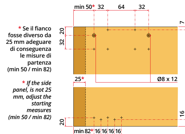
Art. 2007 Fermo superiore in nylon Upper nylon stopper
